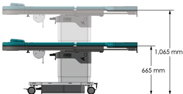
Height Adjustment
