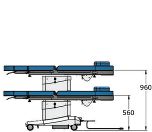
Height Adjustment
