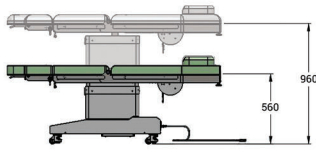
Height Adjustment
