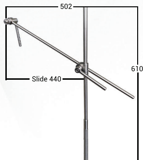
Nathanson Bar Set
